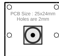
Raspberry Pi Camera Module Mounting Hole Template http://www.raspberrypi-spy.co.uk
